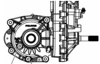
Fill Plug Drain Plug
