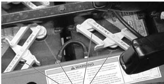
Cell Covers
